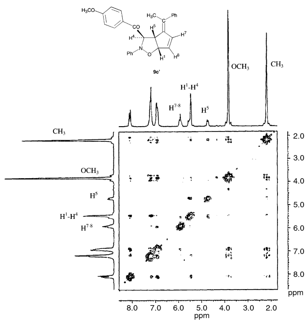
Fig. 1 ^1\text{H} - ^1\text{H} NOESY spectrum of compound 9c' .
